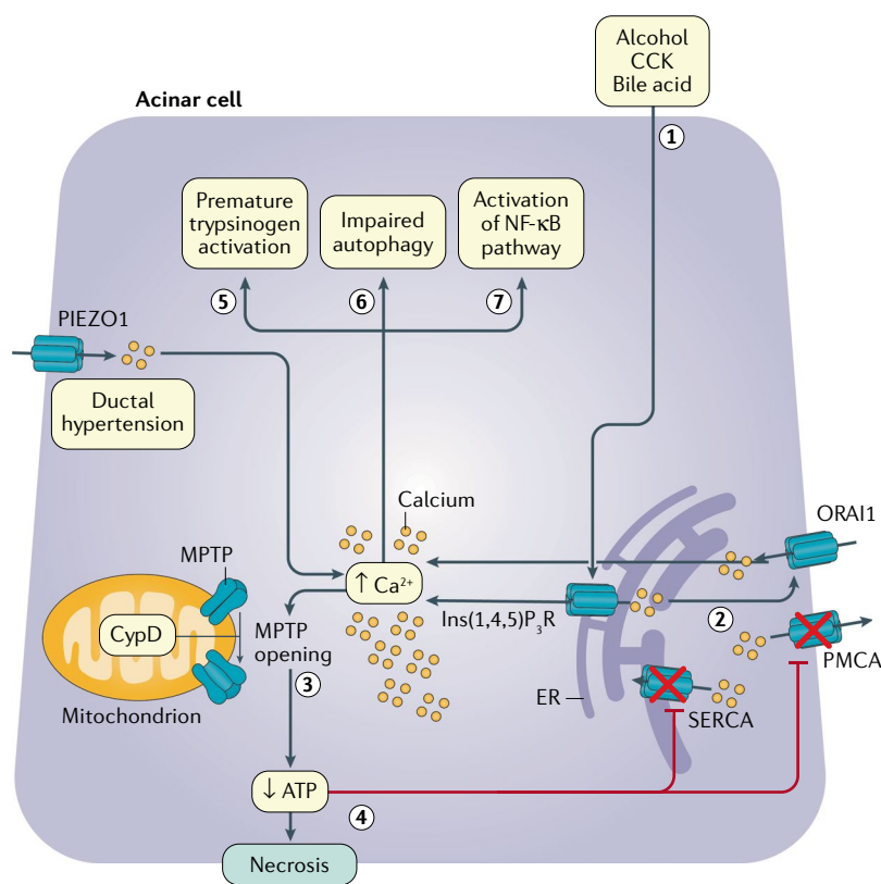
Fig. 1 | Calcium-mediated mitochondrial dysfunction and cell death in acute pancreatitis. In acinar cells, alcohol, cholecystinin (CCK) and bile acid cause inositol 1,4,5-trisphosphate receptor (Ins(1,4,5)P 3 R)-mediated calcium release from the endoplasmic reticulum (ER) (1). The resulting low calcium concentration in the ER triggers opening of calcium release-activated calcium channel protein 1 (ORAI1), through which calcium enters the cell from the extracellular space (2). This results in pathological global calcium concentration elevation. Calcium elevation results in opening of mitochondrial permeability transition pores (MPTPs) to a high-conductance state, and loss of membrane potential across the mitochondrial membrane ensues (3). This process results in mitochondrial dysfunction and necrosis. Mitochondrial dysfunction leads to ATP depletion, which impairs ATP-dependent mechanisms to reduce cytosolic calcium (4). This process then accentuates and perpetuates the pathological calcium toxicity. Pathological calcium elevation also causes other cytotoxic pathways (5), including premature trypsinogen activation, autophagy impairment (6) and activation of the nuclear factor- \kappa B (NF- \kappa B) pathway (7). The NF- \kappa B pathway leads to production of pro-inflammatory mediators. The PIEZO1 mechanoreceptor, which contains cation channel properties and is activated by pressure, also promotes increased calcium entry from outside the acinar cell (8). CypD, cyclophilin D; PMCA: plasma membrane Ca 2+ channel; SERCA, smooth ER Ca 2+ channel.
